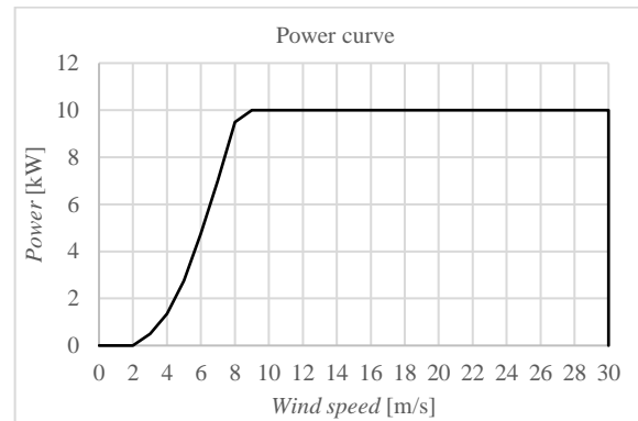
Figure 6. Wind turbine power curve
