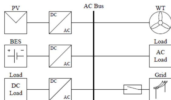
Figure 2. The topology of the DC microgrid
