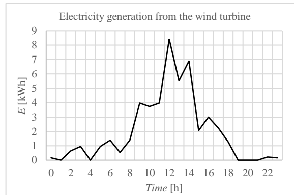
Figure 10. Electricity generation from wind turbine
