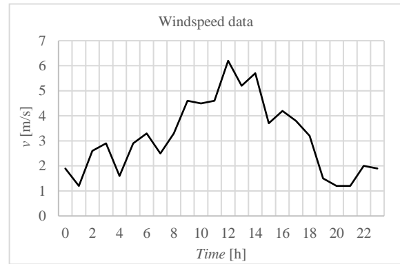
Figure 5. Wind speed data
