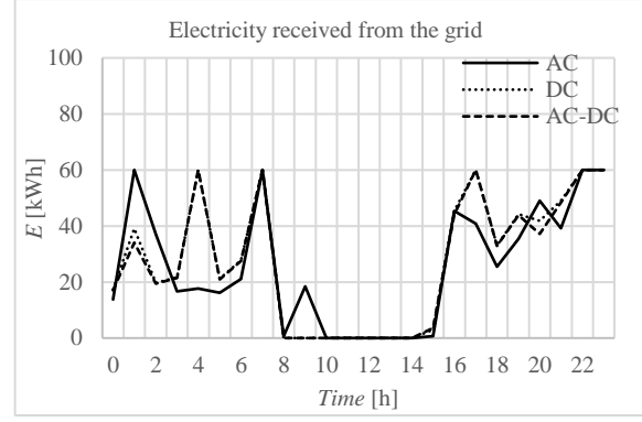
Figure 15. Comparison of electricity received from grid for AC, DC and hybrid AC-DC microgrid
