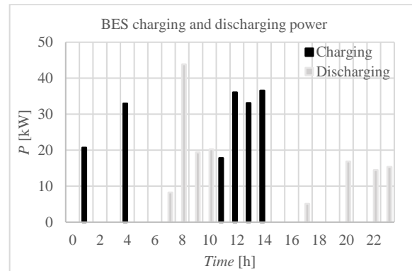
Figure 12. Charging and discharging power of BES in DC microgrid
